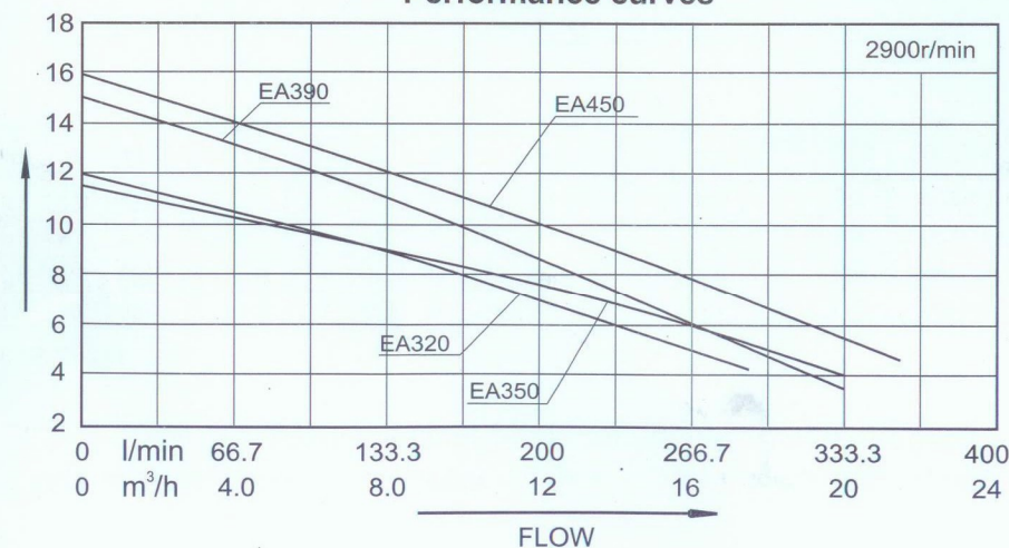
Performance curves
